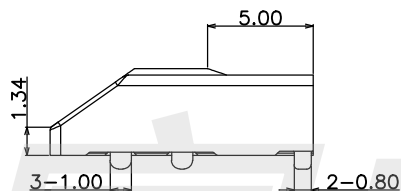
PLUG MATE DRAWING
