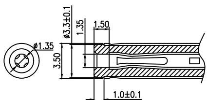
MATE PLUG
