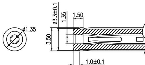
MATE PLUG
