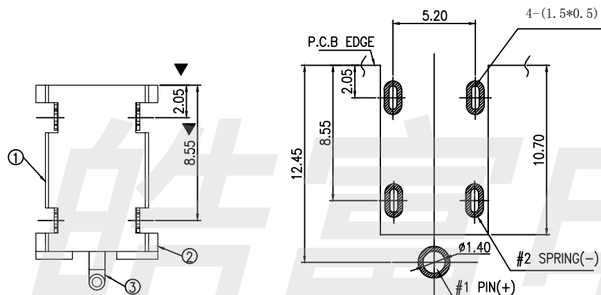
RECOMMENDED PCB LAYOUT TOP VIEW (TOLERANCE:±0.05)
