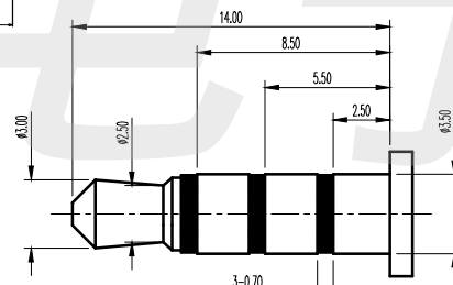
(Ø3.50mm 4 POLE PLUG DETAIL DRAWING)
