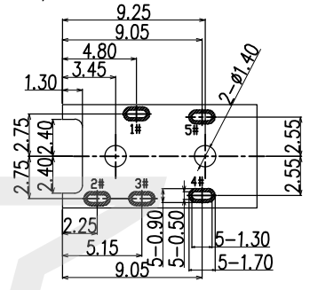
P.C.B LAYOUT T=1.00mm TOP VIEW
