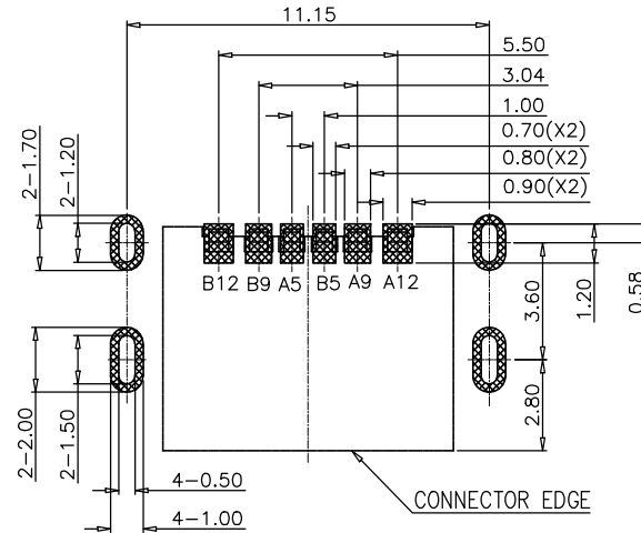
RECOMMENDED PCB LAYOUT(TOP VIEW) THICKNESS 1.6±0.10MM;DEFAULT TOLERANCE:±0.05
