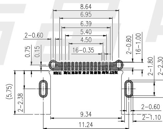
RECOMMENDED PCB LAYOUT General Tolerance ±0.05mm
