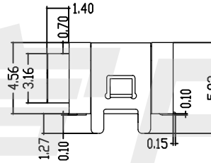
RECOMMENDED P.C.B. LAYOUT TOLERANCE UNSPECIFIED ±0.05mm
