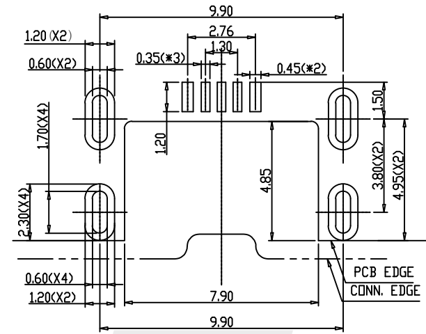
RECOMMENDED PCB LAYOUT(TOP VIEW) GENERAL TOLERANCES:±0.05
