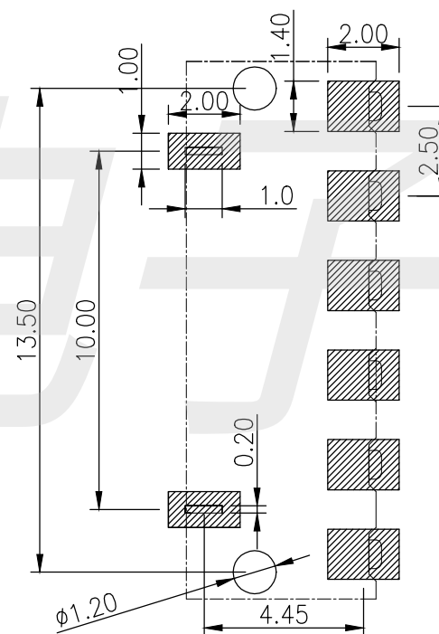
RECOMMENDED PCB LAYOUT TOP VIEW(.XX±0.05)
