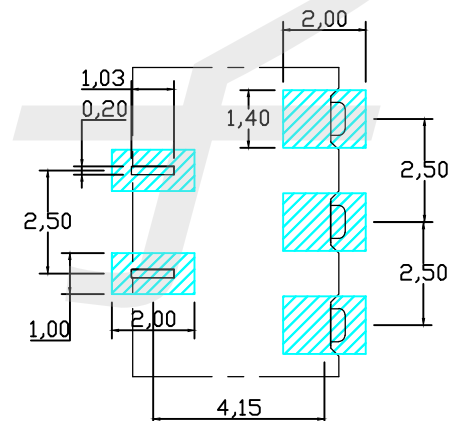
RECOMMENDED PCB LAYOUT TOP VIEW (.XX ± 0.05)
