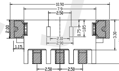
PCB LAYOUT (3pin)
