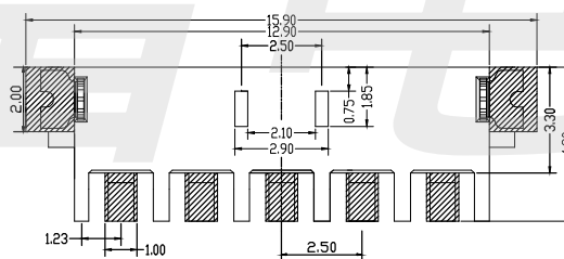
PCB LAYOUT (5pin)
