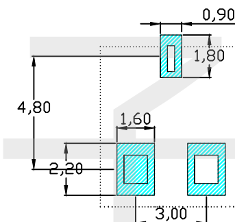
RECOMMENDED PCB LAYOUT TOP VIEW (.XX±0.05)
