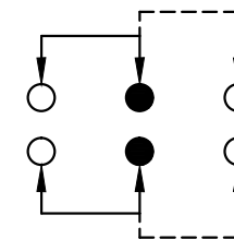
SCHEMATIC (NON-SHORTING)
