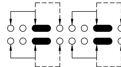
SCHEMATIC (NON-SHORTING)
