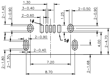
RECOMMENDED P.C.B. LAYOUT (TOP VIEW) GENERAL TOLERANCE: \pm 0.05
