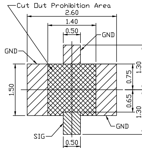
RECOMMENDED P.C.B. LAYOUT TOP VIEW (TOLERANCE: \pm 0.05 )
