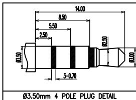
0.35mm 4 POLE PLUG DETAIL
