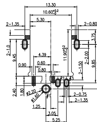
PCB LAYOUT TOP VIEW TOLERANCES:±0.05
