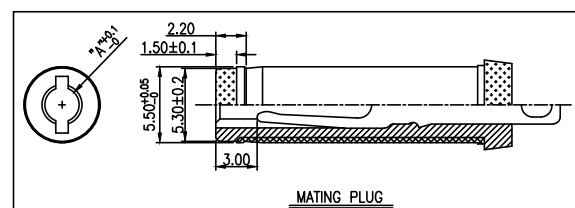
MATING PLUG
