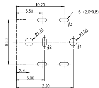
PCB LAYOUT TOP VIEW TOLERANCES:±0.05
