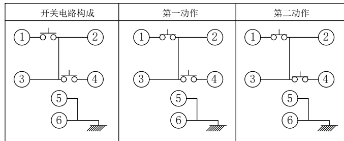
CIRCUIT DIAGRAM
