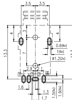
Recommended PCB Layout(T=1.2) Tolerance: ±0.05(TOP view)
